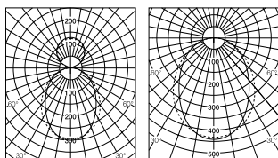
40 W LED, 1216 lm
